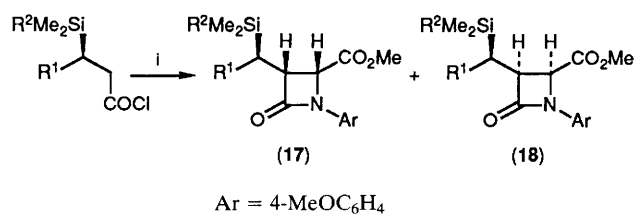
Scheme 2. Reagents and conditions: i, (9a), hexane or MeCN, reflux, 14 h. J_{1',3}(\text{anti}) > J_{1',3}(\text{syn}) .
